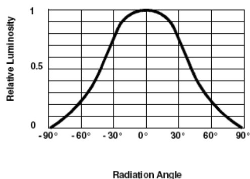
Fig 6. Relative Luminous Intensity vs. Radiation Angle
