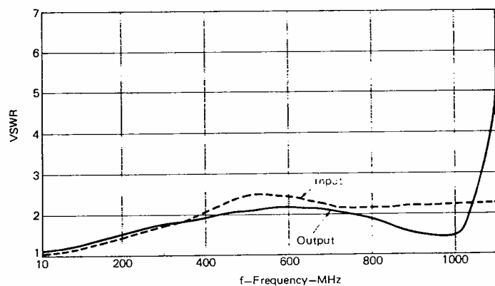
VSWR vs. FREQUENCY
