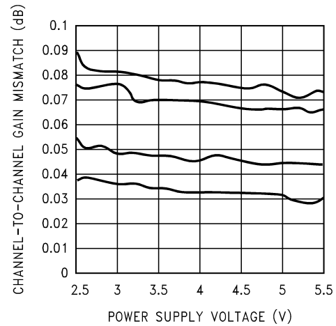
Channel-to-Channel gain Mismatch vs Power Supply Voltage
