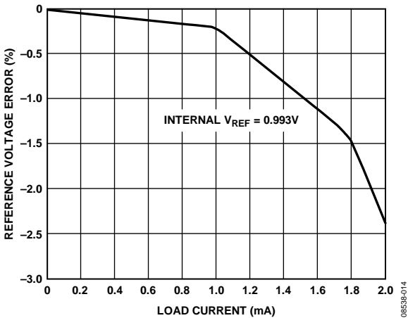
Figure 46. V_{REF} Accuracy vs. Load Current
