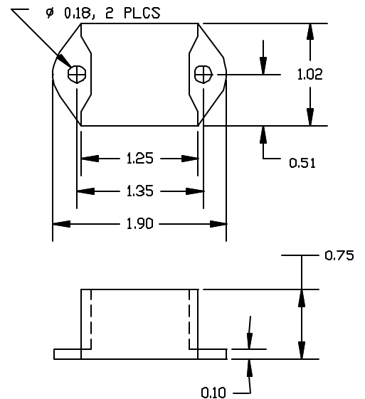
E Package
