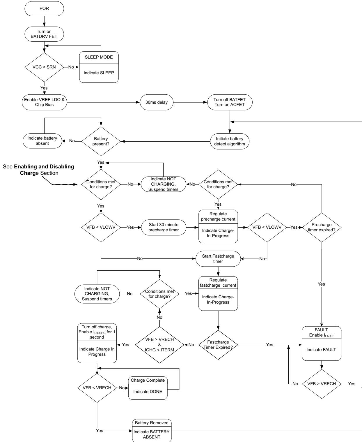
Figure 14. Operational Flowchart
