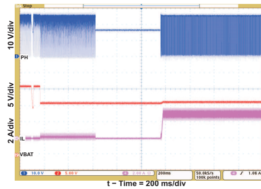
Figure 9. Battery Insertion
