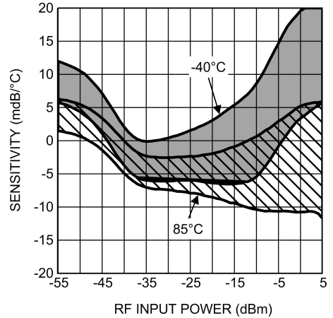
Temperature Sensitivity (Mean ±3 sigma) vs. RF Input Power at 50 MHz
