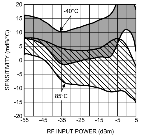
Temperature Sensitivity (Mean ±3 sigma) vs. RF Input Power at 3000 MHz
