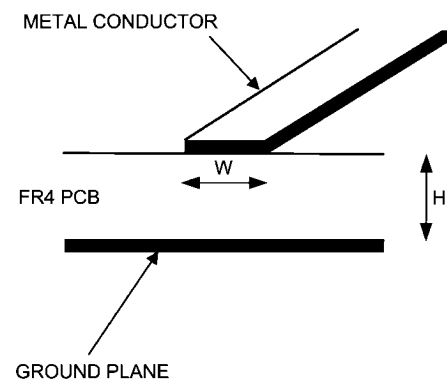
FIGURE 15. Microstrip Configuration
