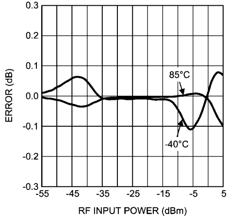
查询"LMH2100"供应商 Error for 1 dB Input Power Step vs. RF Input Power at 1855 MHz
