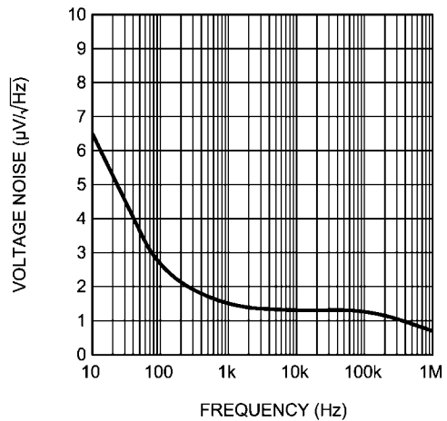
Output Noise Spectrum vs. Frequency
