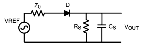
FIGURE 2. Diode Detector
