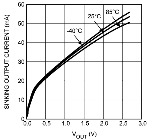
Sinking Output Current vs. Output Voltage
