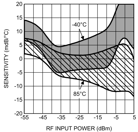
Temperature Sensitivity (Mean ±3 sigma) vs. RF Input Power at 1855 MHz
