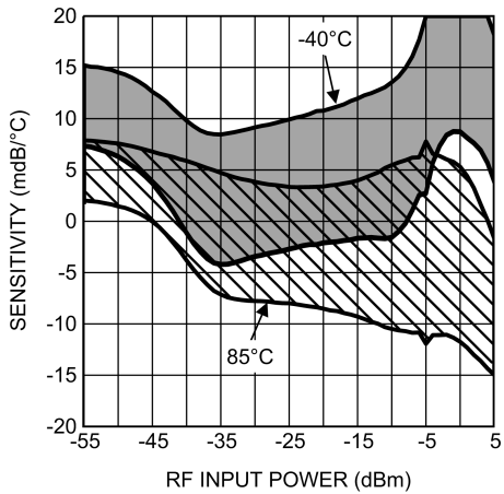
Temperature Sensitivity (Mean ±3 sigma) vs. RF Input Power at 2500 MHz
