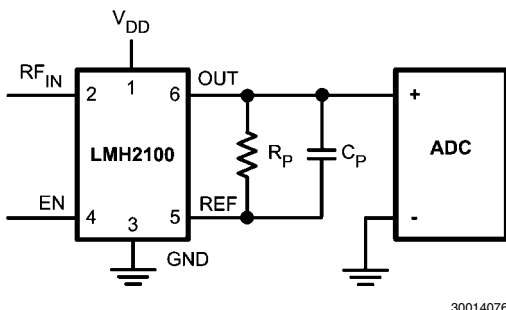
FIGURE 12. Single Ended and Differential Application
