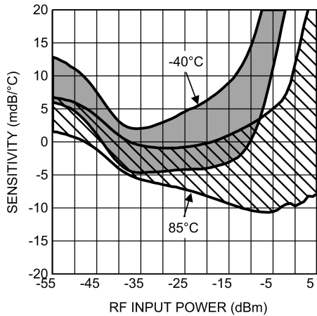
Temperature Sensitivity (Mean ±3 sigma) vs. RF Input Power at 900 MHz
