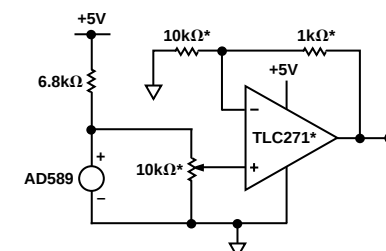
Figure 19. Reference Adjust Circuit
