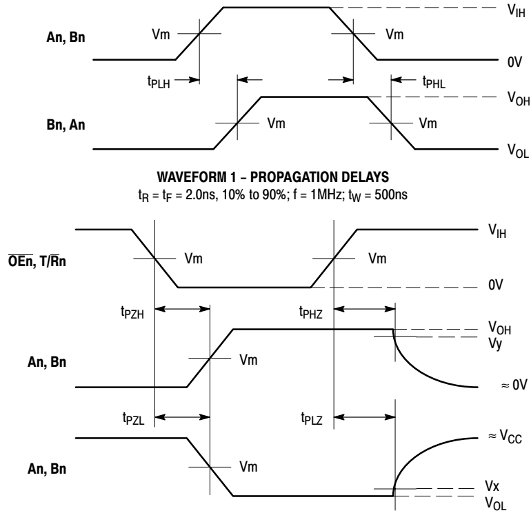
Figure 4. AC Waveforms
