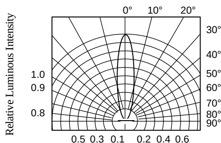
FIG.6 RADIATION DIAGRAM
