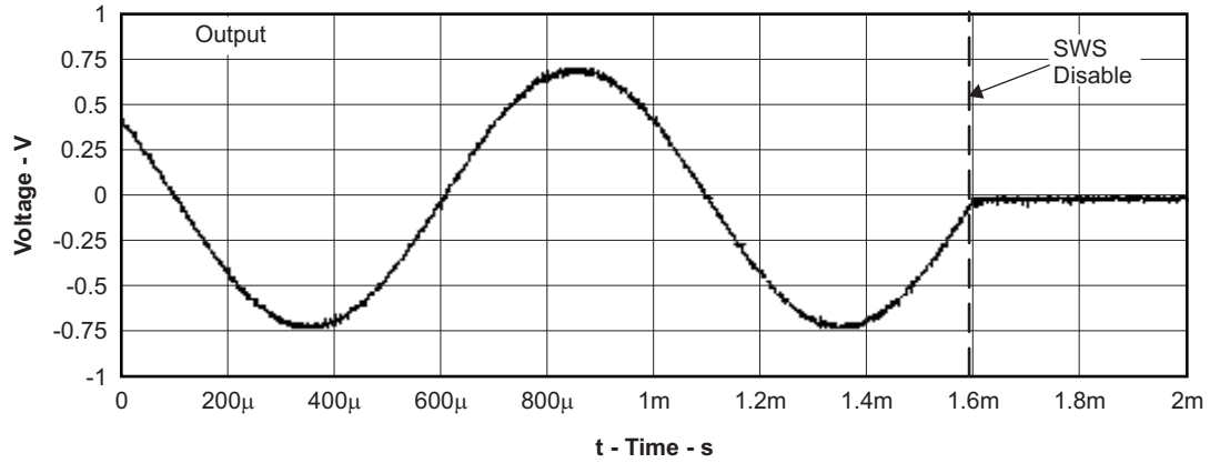
Figure 29. Shutdown Time
