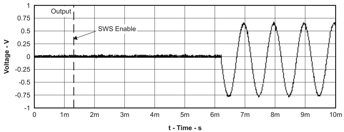
Figure 30. Startup Time
