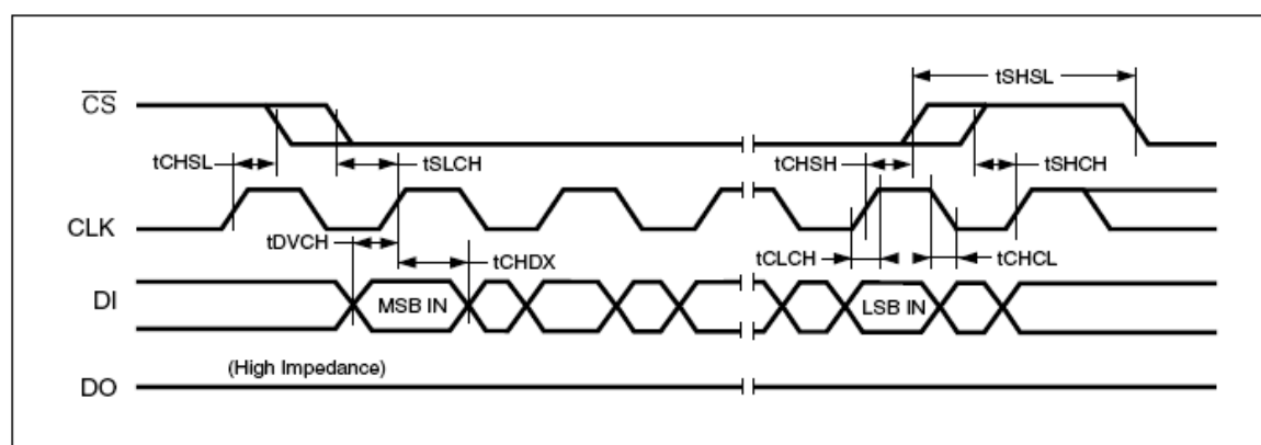
Figure 24. Input Timing
