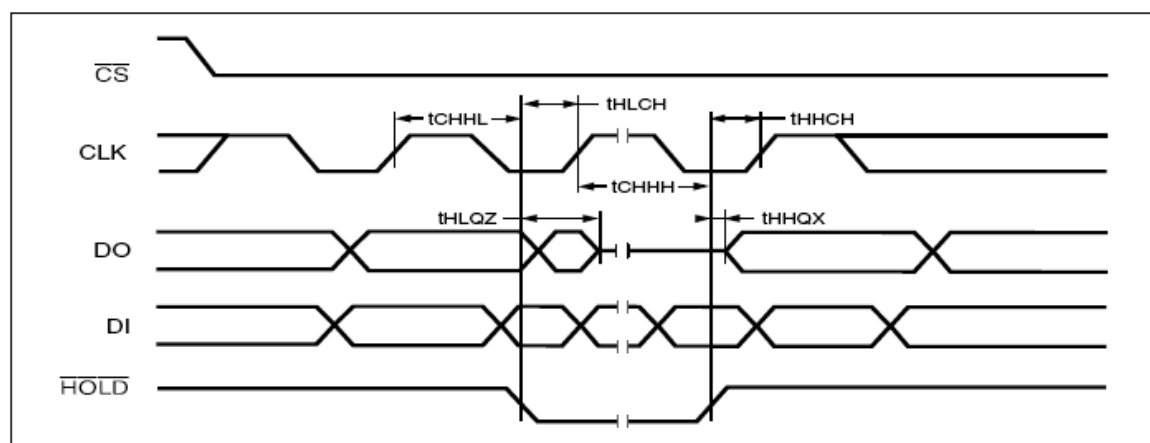
Figure 25. Hold Timing
