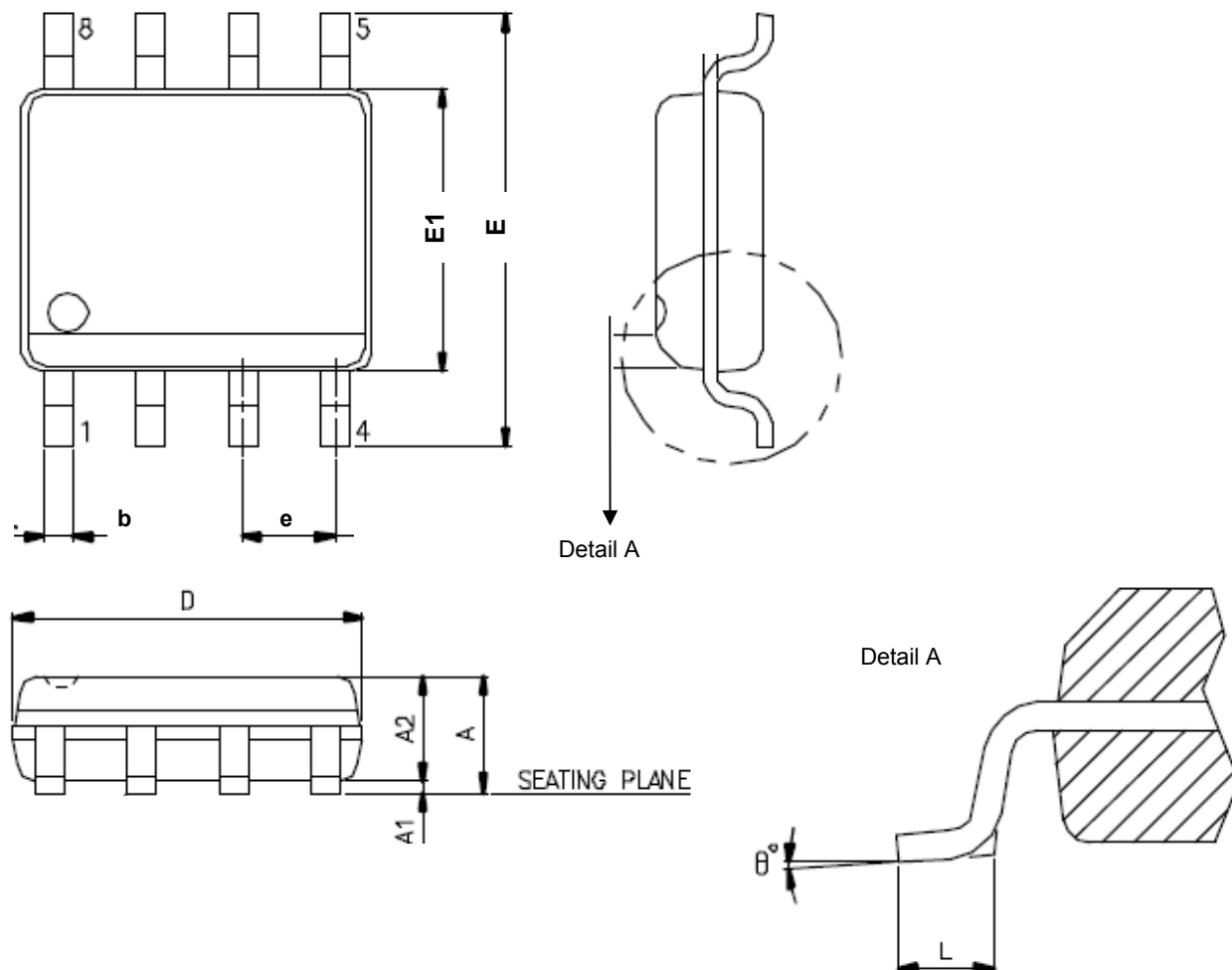
Figure 26. SOP 8 ( 150 mil )
