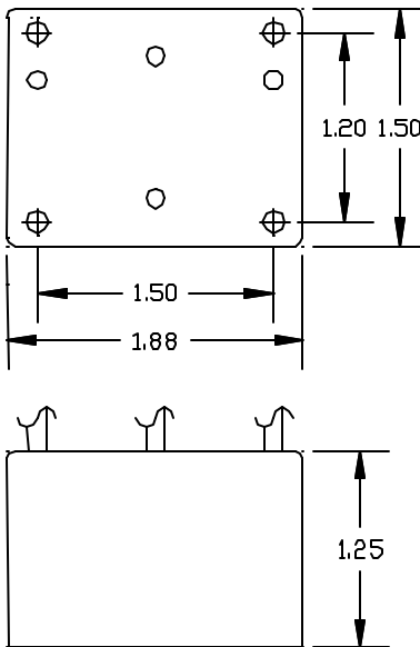
D Package
