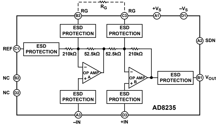
Figure 35. Simplified Schematic
