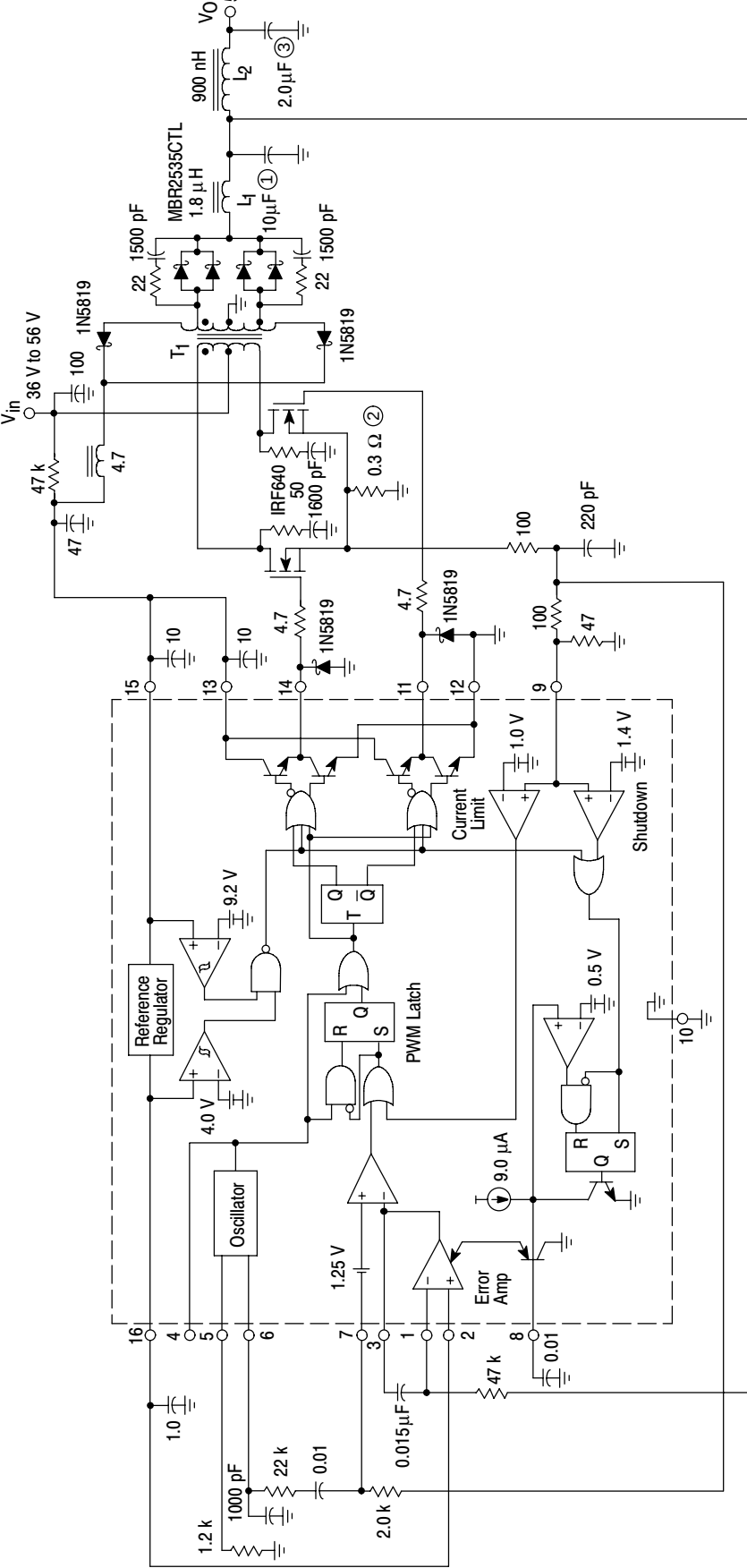
Figure 37. Application Circuit
