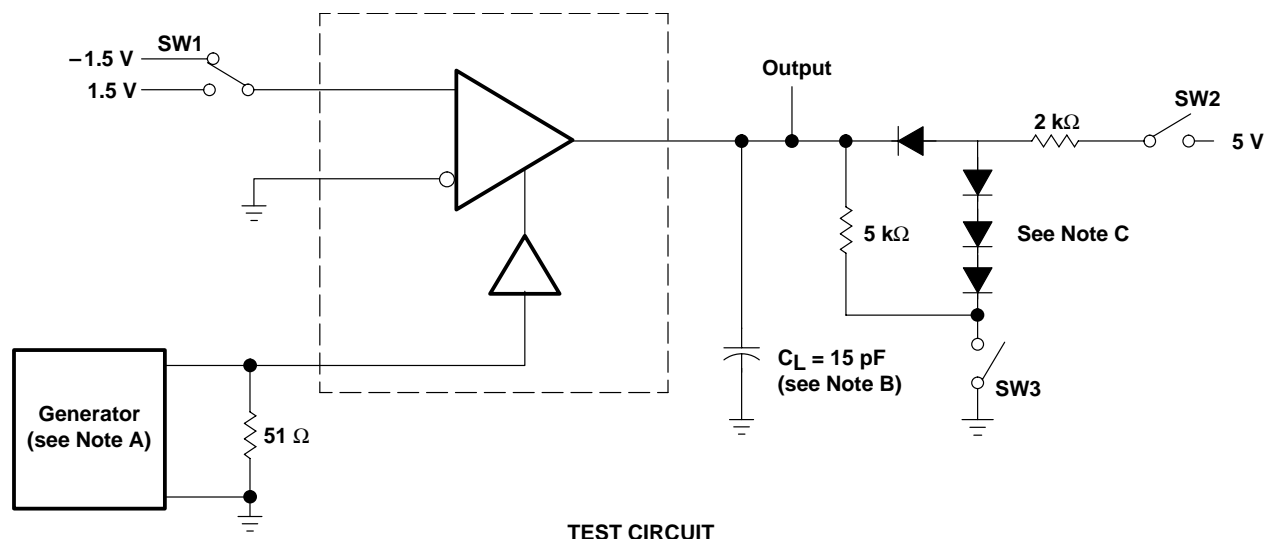
TEST CIRCUIT
