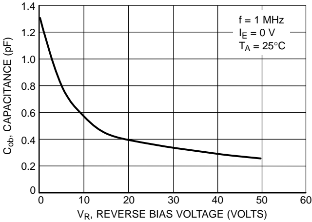
Figure 36. Output Capacitance
