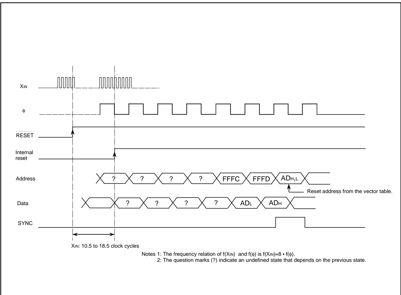
Fig. 53. Reset sequence
