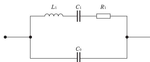
Equivalent electric circuit of a quartz crystal unit
