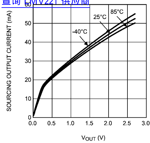
Sourcing Output Current vs. Output Voltage
