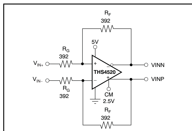
Figure 41. Basic Differential Input Signal Interface
