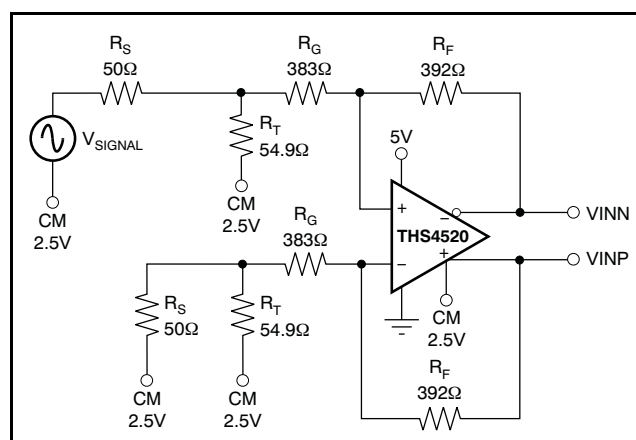
Figure 42. Basic Single-Ended Input Signal Interface
