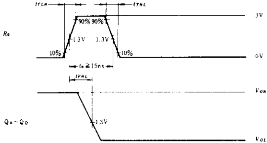
Waveform-3 t_{PLH} , t_{PHL}(R_9 \rightarrow Q)
