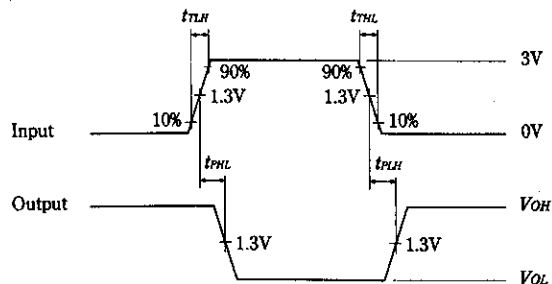
Waveform
