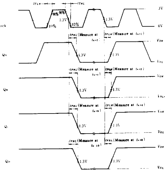
Waveform-1 f_{max} , t_{PLH} , t_{PHL} (Clock \rightarrow Q)
