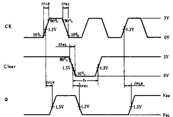
Waveform-2 (Clear→Q)
