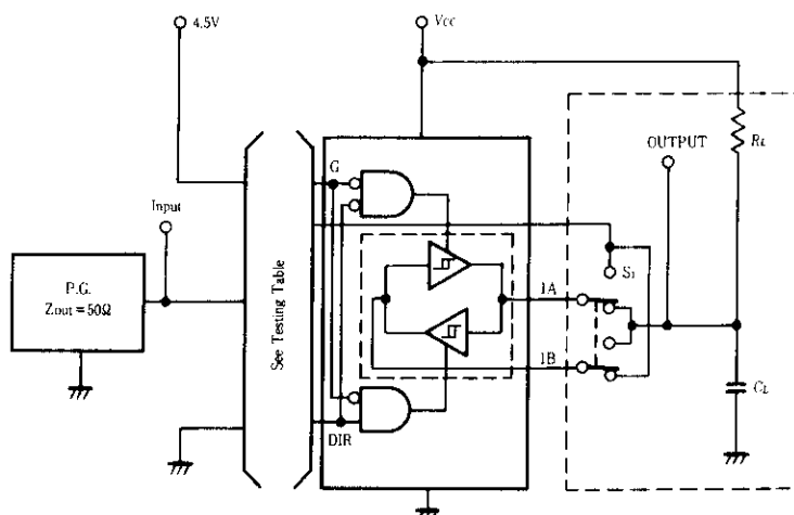
Test Circuit
