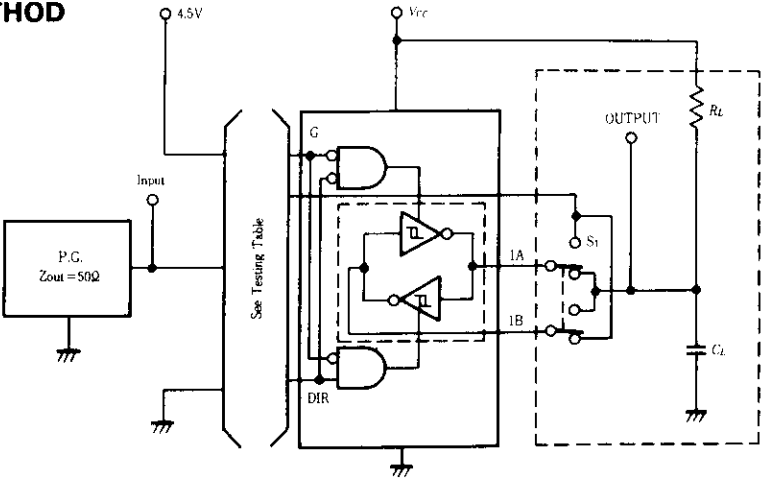
Test Circuit
