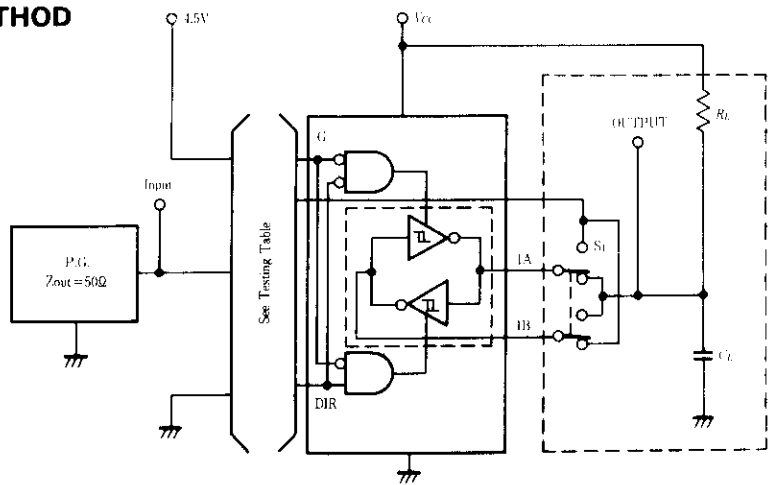
Test Circuit
