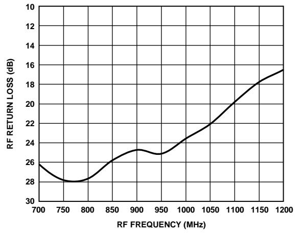
Figure 31. RF Return Loss, Fixed IF
