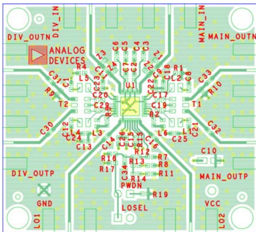
Figure 55. Evaluation Board Top Layer
