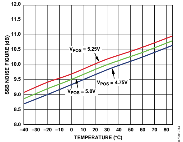
Figure 14. SSB Noise Figure vs. Temperature
