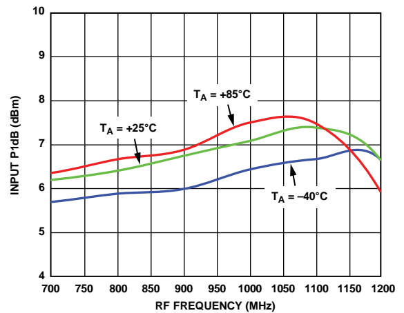
Figure 50. Input P1dB vs. RF Frequency at 3.3 V
