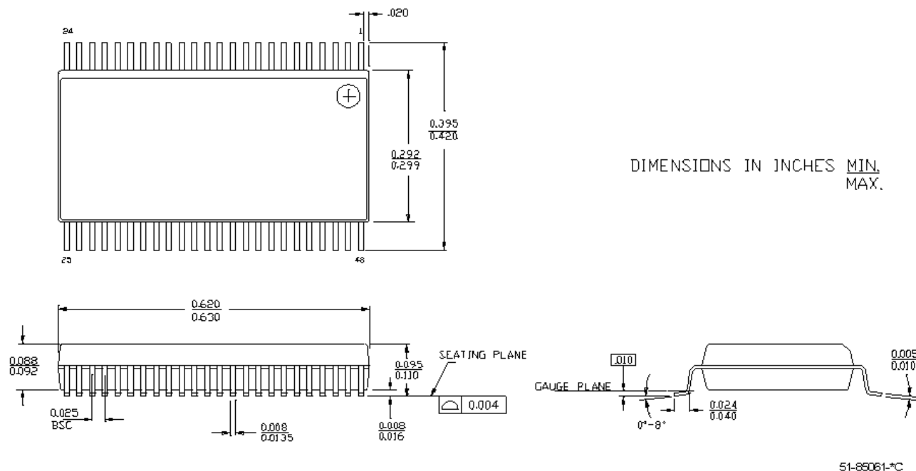
Figure 19. 48-Pin SSOP (51-85061)
