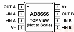
Figure 4. AD8666, 8-Lead MSOP (RM-8)
