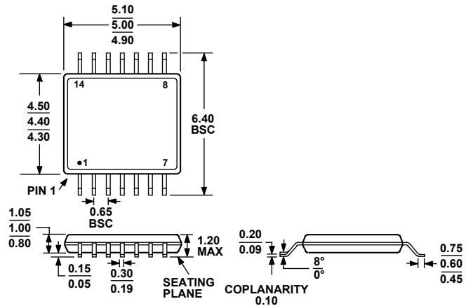
Figure 43. 14-Lead Thin Shrink Small Outline Package [TSSOP] (RU-14)
