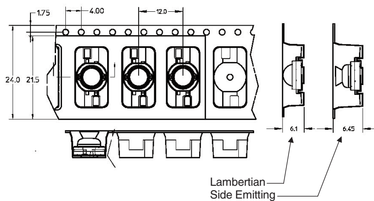
Figure 9. Tape dimensions.
