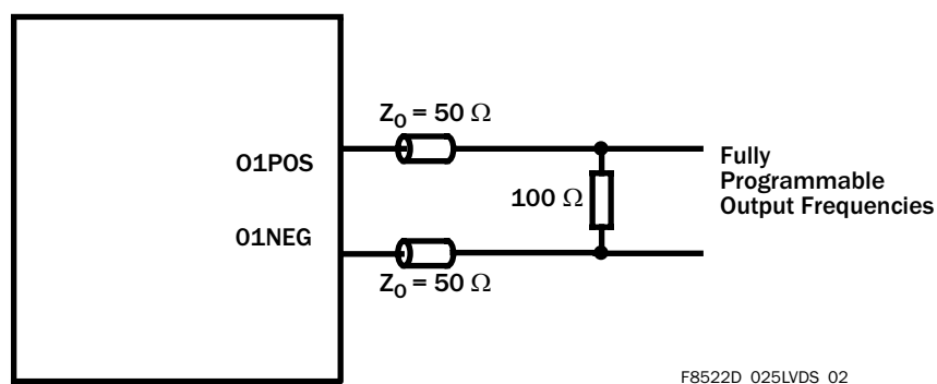
Figure 11 Recommended Line Termination for LVDS Output Port
