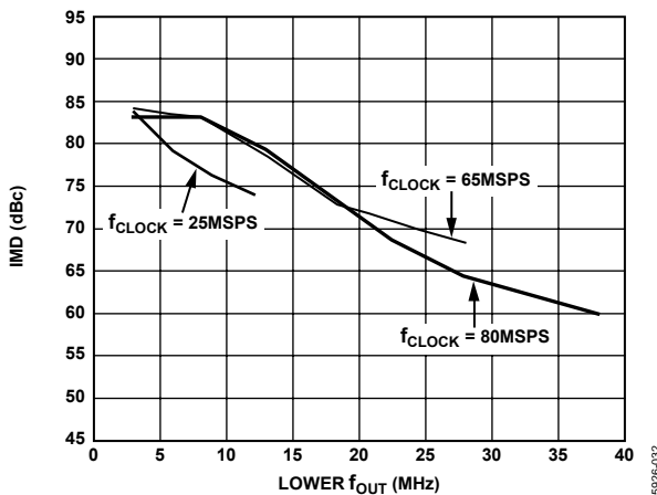
Figure 35. Dual-Tone IMD vs. Lower f_{OUT} @ I_{OUTFS} = 2\text{mA} and 0 dBFS
