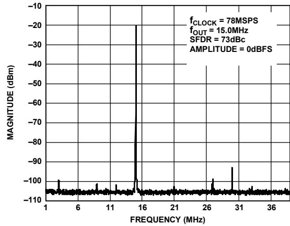
Figure 68. AD9706 Single-Tone SFDR
