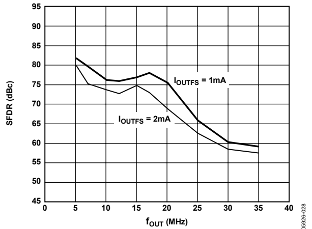
Figure 31. SFDR vs. f_{OUT} and I_{OUTFS} @ 80 MSPS
