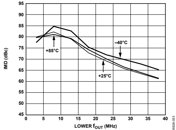
Figure 36. Dual-Tone IMD vs. Lower f_{OUT} and Temperature @ 80 MSPS, I_{OUTFS} = 1\text{mA} and 0 dBFS
