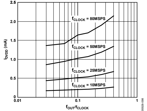
Figure 84. I_{DVDD} vs. f_{OUT}/f_{CLOCK} Ratio @ DVDD = 1.8 V
