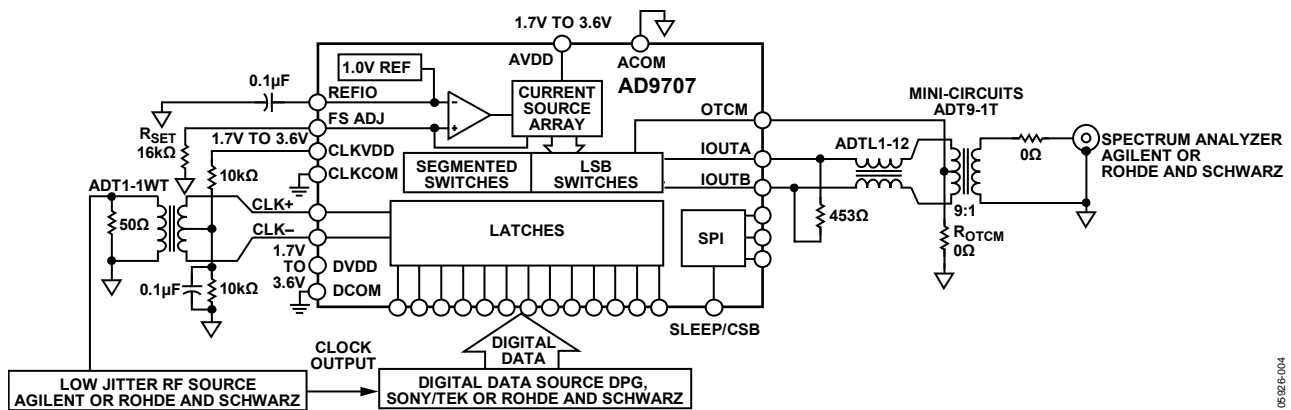
Figure 70. Basic AC Characterization Test Setup
