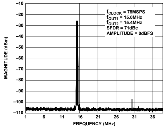
Figure 67. AD9705 Dual-Tone SFDR
