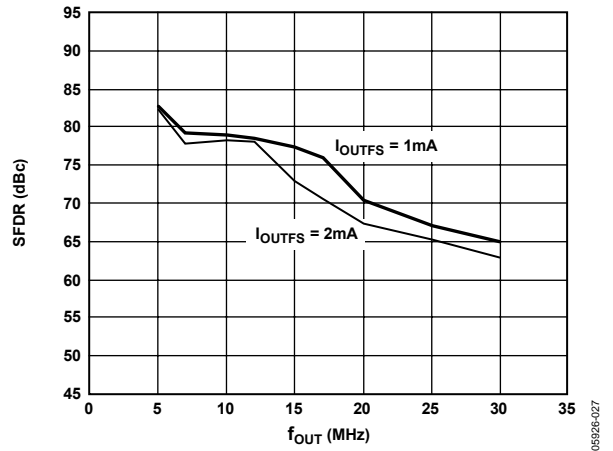
Figure 30. SFDR vs. f_{OUT} and I_{OUTFS} @ 65 MSPS
