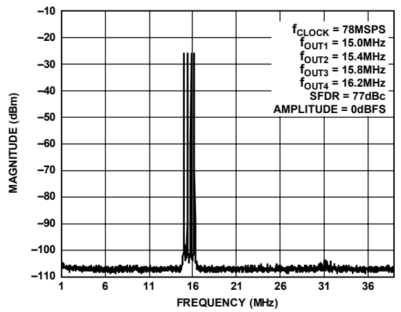
Figure 43. Four-Tone SFDR
