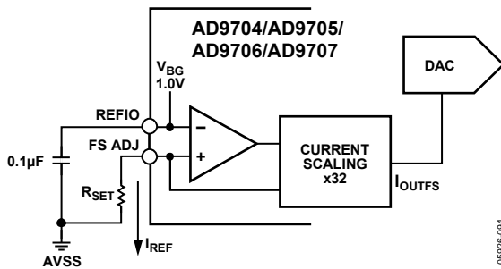
Figure 78. Internal Reference Configuration
