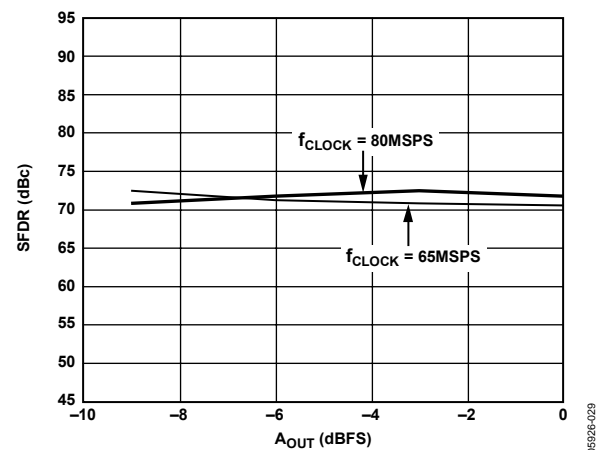
Figure 32. SFDR vs. A_{OUT} @ f_{OUT} = f_{CLOCK}/5
