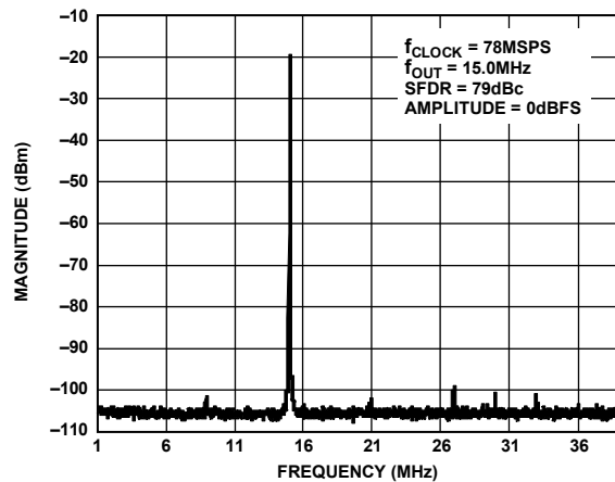
Figure 24. Single-Tone SFDR
