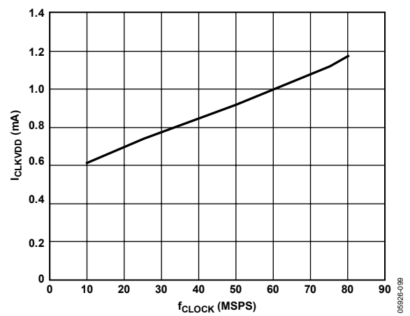
Figure 86. I_{CLKVDD} vs. f_{CLOCK} (Differential Clock Mode) @ CLKVDD = 1.8 V
