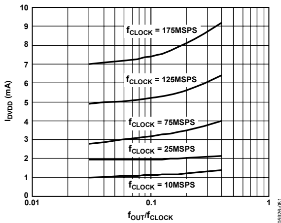
Figure 83. I_{DVDD} vs. f_{OUT}/f_{CLOCK} Ratio @ DVDD = 3.3 V
