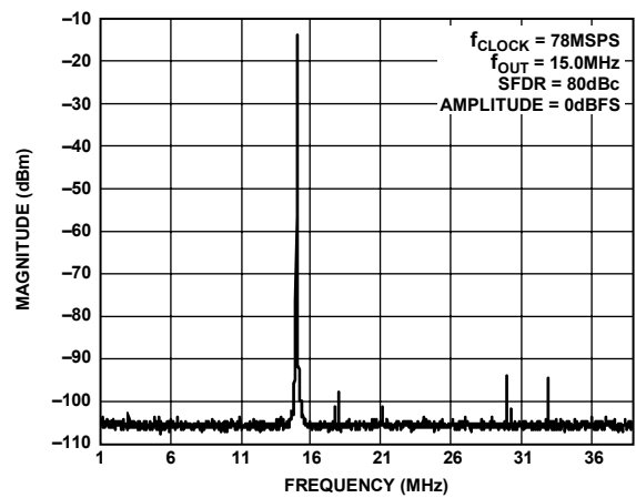
Figure 41. Single-Tone SFDR
