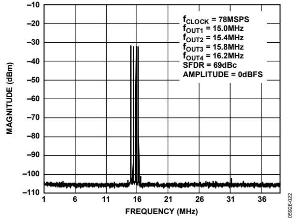
Figure 26. Four-Tone SFDR
