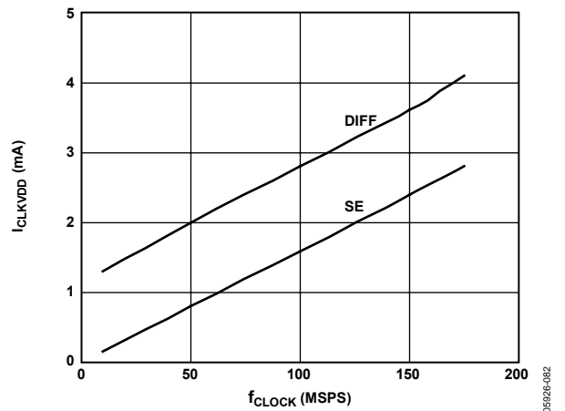
Figure 85. I_{CLKVDD} vs. f_{CLOCK} @ CLKVDD = 3.3 V
