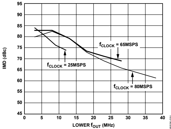
Figure 34. Dual-Tone IMD vs. Lower f_{OUT} @ I_{OUTFS} = 1\text{mA} and 0 dBFS
