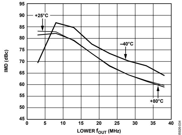
Figure 37. Dual-Tone IMD vs. Lower f_{OUT} and Temperature @ 80 MSPS, I_{OUTFS} = 2\text{mA} and 0 dBFS
