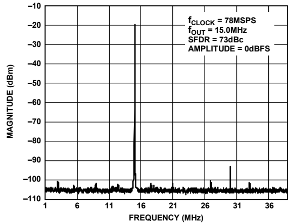
Figure 66. AD9705 Single-Tone SFDR
