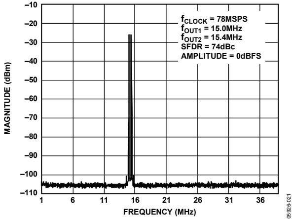
Figure 25. Dual-Tone SFDR
