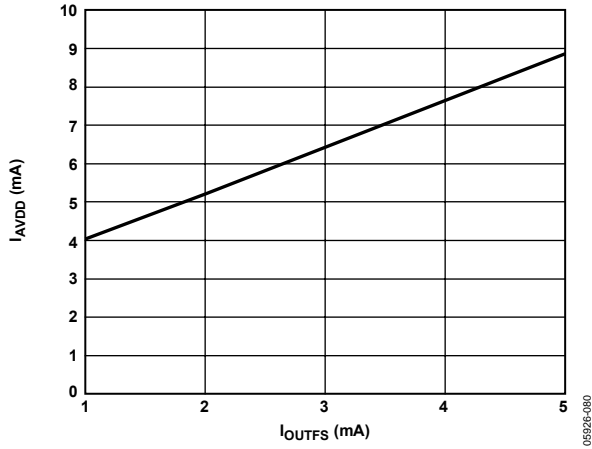
Figure 81. I_{AVDD} vs. I_{OUTFS} @ AVDD = 3.3 V
