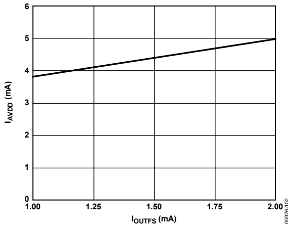
Figure 82. I_{AVDD} vs. I_{OUTFS} @ AVDD = 1.8 V
