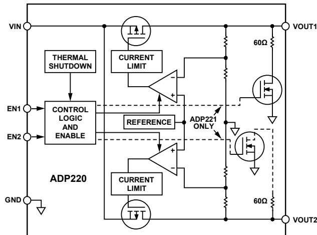
Figure 28. Internal Block Diagram
