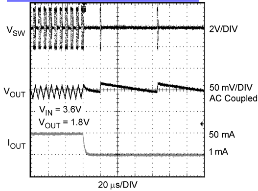
Load Transient Response ( V_{OUT} = 1.8V ) 查询"LM3679" (共 5 页)
