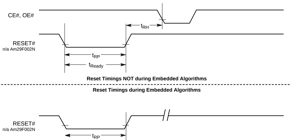
Figure 10. RESET# Timings
