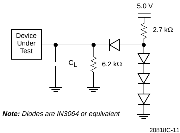
Figure 8. Test Setup
