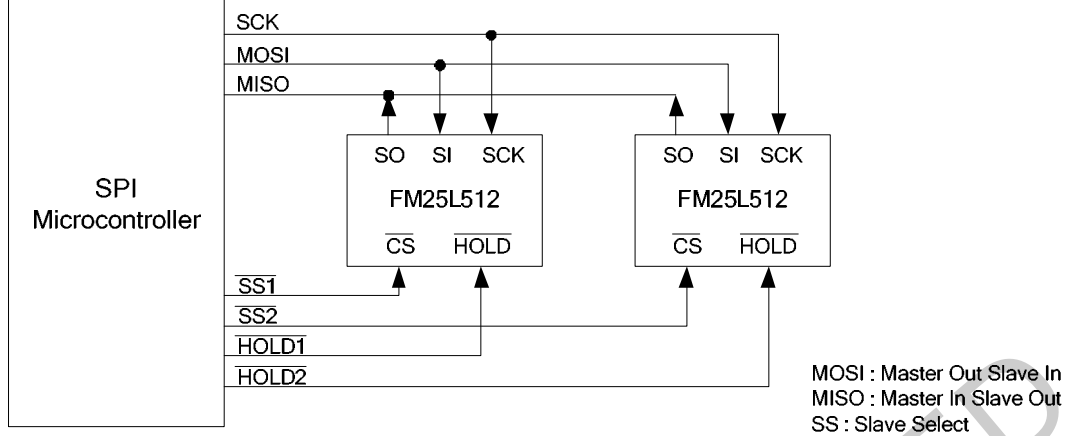
Figure 2. 1Mbit System Configuration with SPI port
