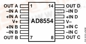
Figure 5. 14-Lead TSSOP (RU Suffix)
