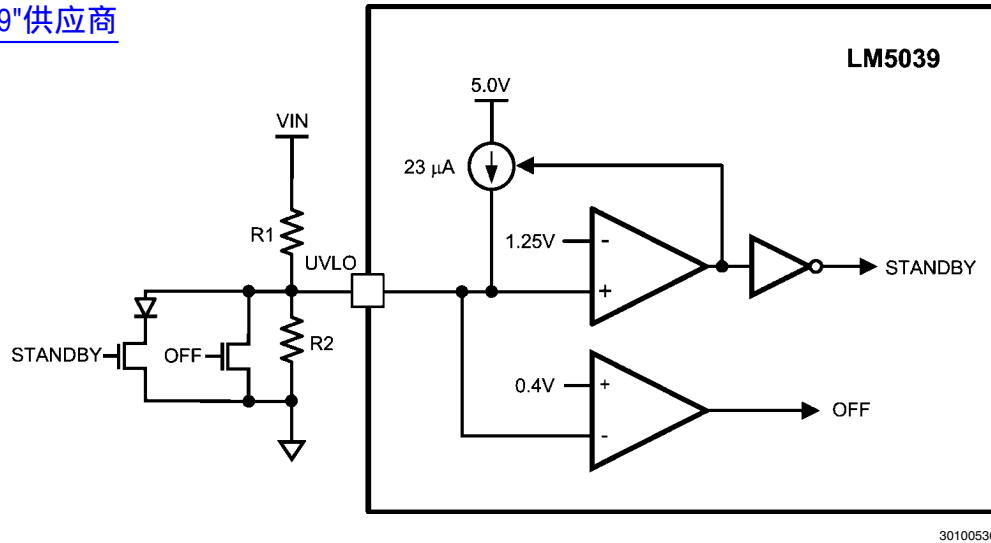
FIGURE 11. Remote Disable and Control
