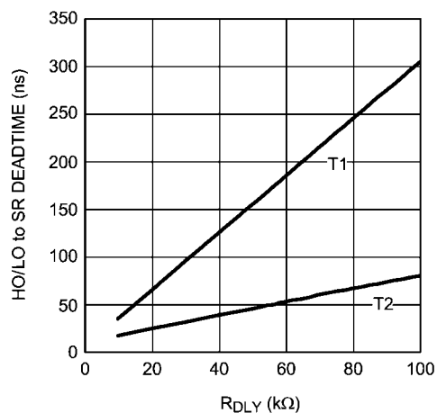
R_{\text{DLY}} vs SR Deadtime
