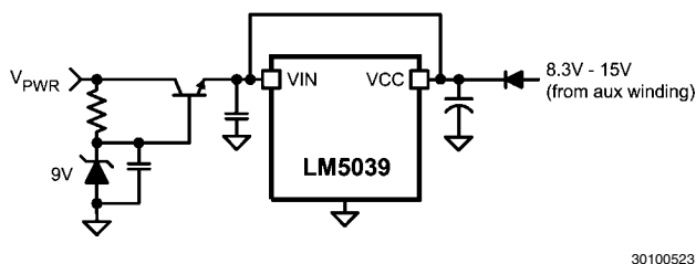
FIGURE 7. Start-up Regulator for V_{PWR} > 100V
