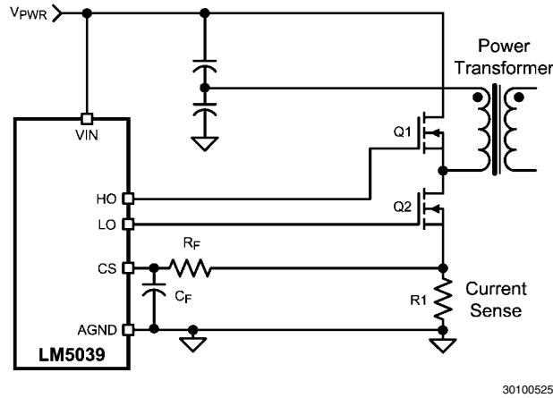
FIGURE 9. Current Sense Using Current Sense Resistor (R1)
