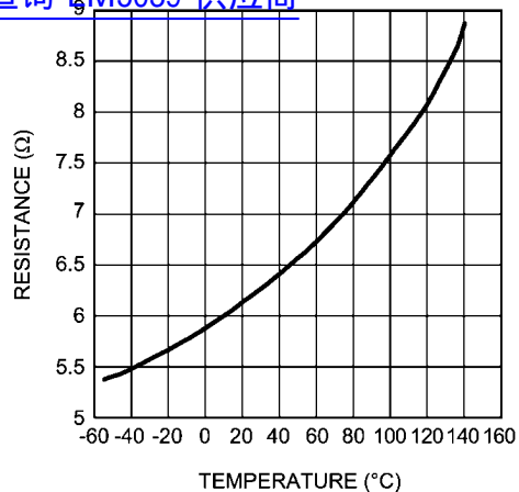
Effective Comp Input Impedance 查询"LM5039"供应商
