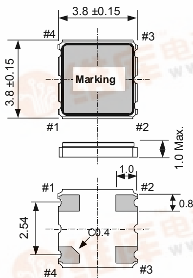
Pin map
