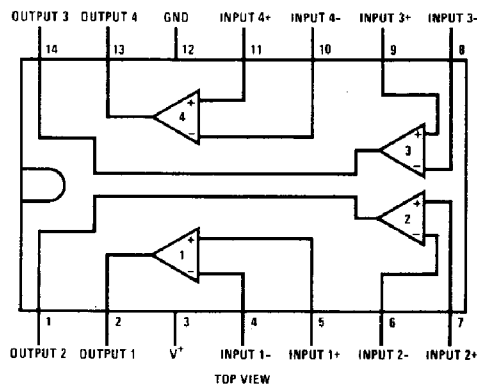
Dual-In-Line Package
