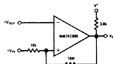
Non-Inverting Comparator with Hysteresis
