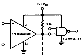
Driving CMOS
