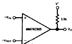
Basic Comparator
