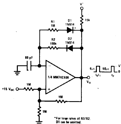
Pulse Generator
