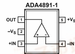
Figure 2. 5-Lead SOT-23 (RJ-5)
