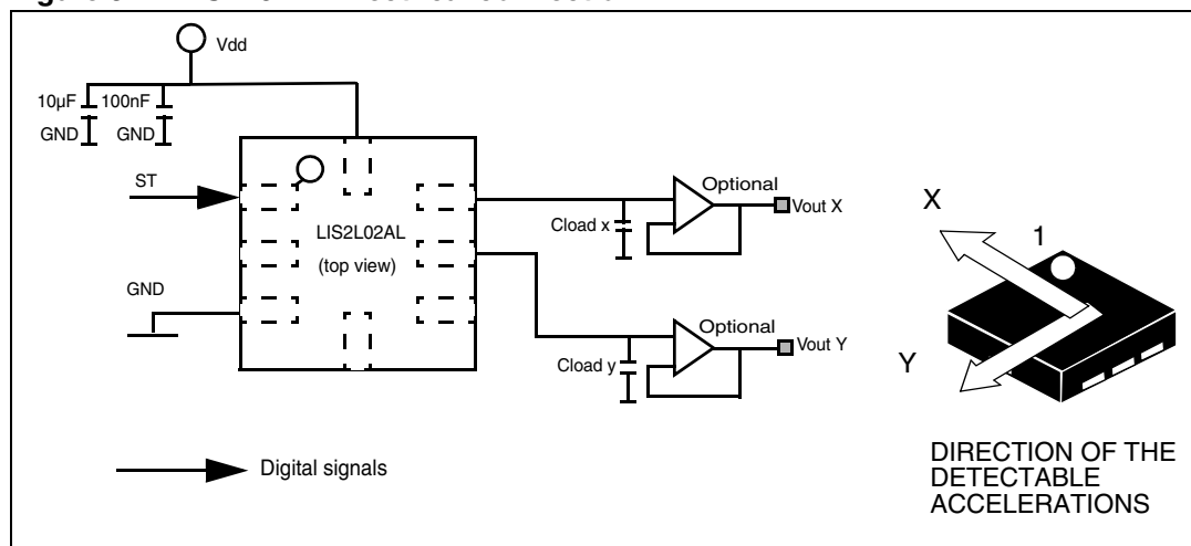
Figure 3. LIS2L02AL Electrical connection
