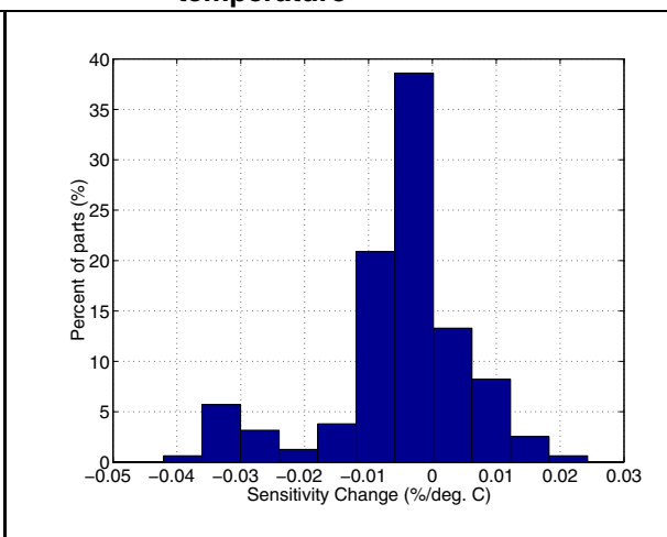
Figure 12. y-axis sensitivity change Vs temperature
