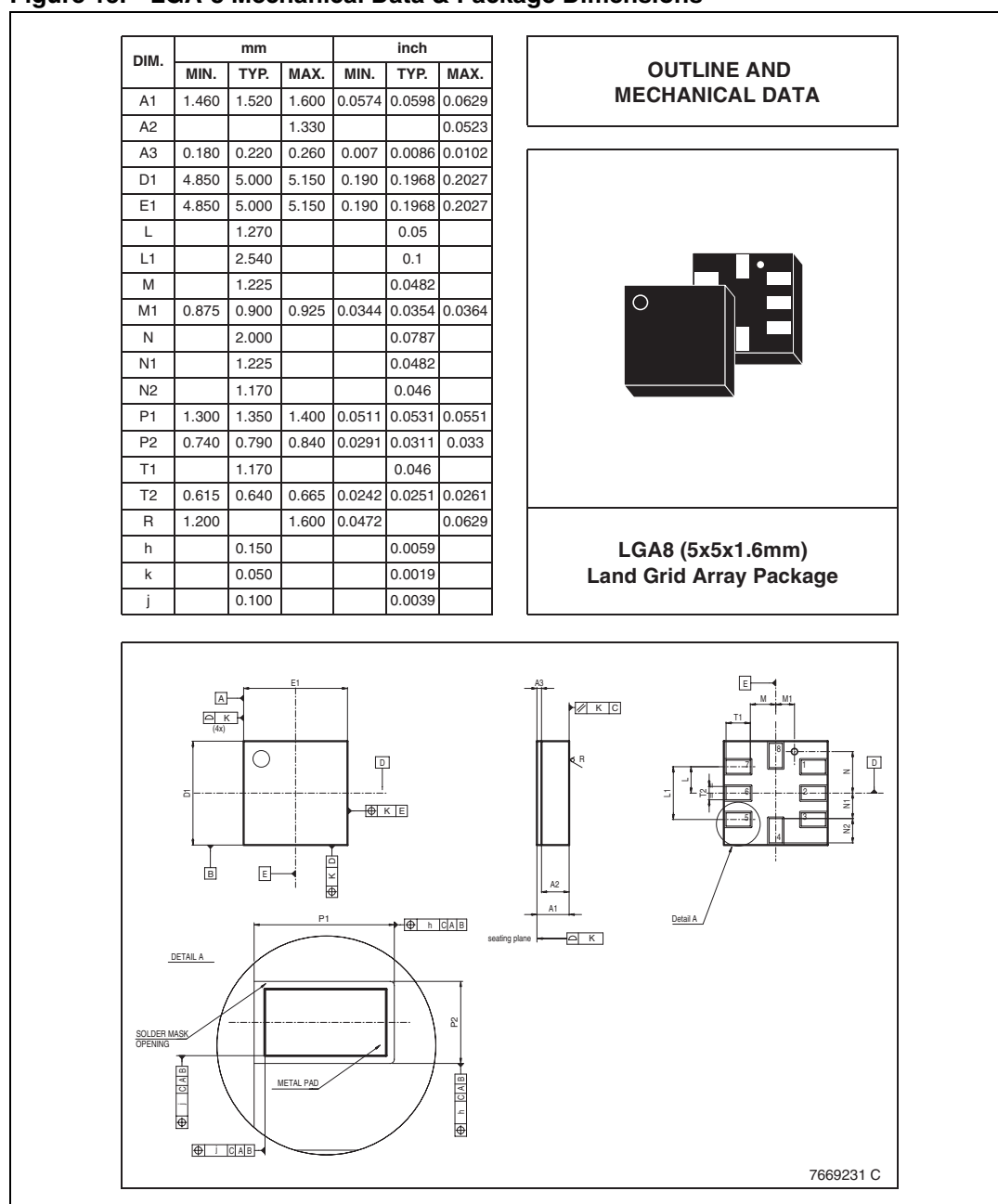
Figure 15. LGA-8 Mechanical Data & Package Dimensions
