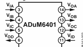
Figure 3. ADuM6401
