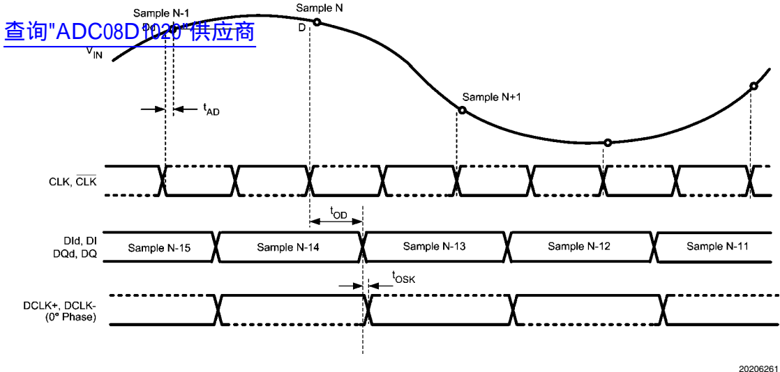
FIGURE 5. ADC08D1020 Timing — DDR Clocking in Non-Demultiplexed and Normal Mode
