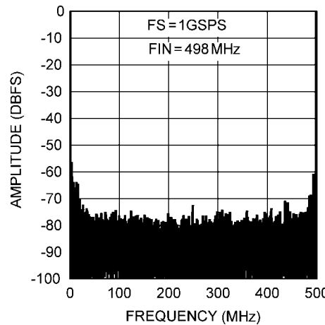
SPECTRAL RESPONSE AT f_{IN} = 498 MHz
