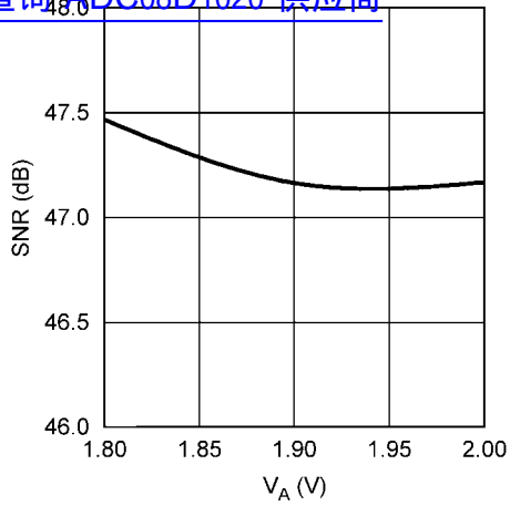
SNR vs. SUPPLY VOLTAGE 查询"ADC08D1020"供应商
