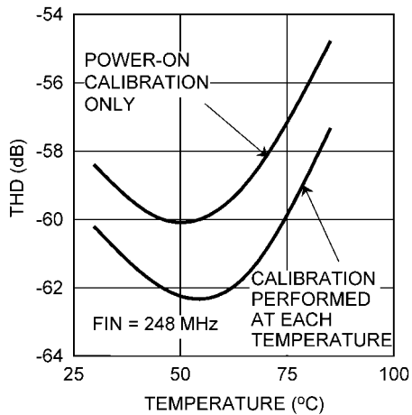
THD vs. DIE TEMPERATURE
