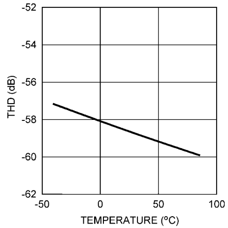
THD vs. AMBIENT TEMPERATURE
