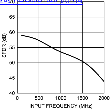
SFDR vs. INPUT FREQUENCY 查询"ADC08D1020"供应商
