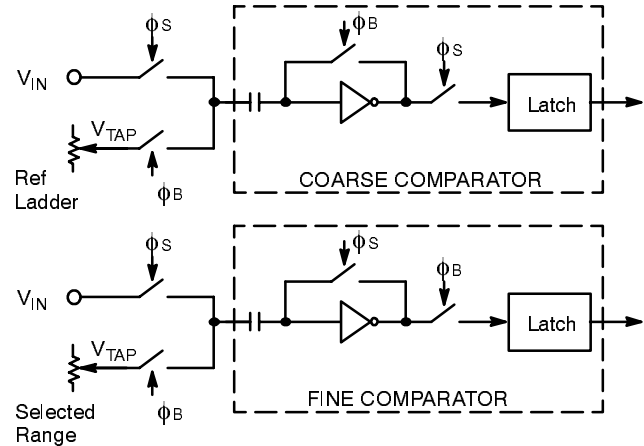
Figure 2. MP8795 Comparators
