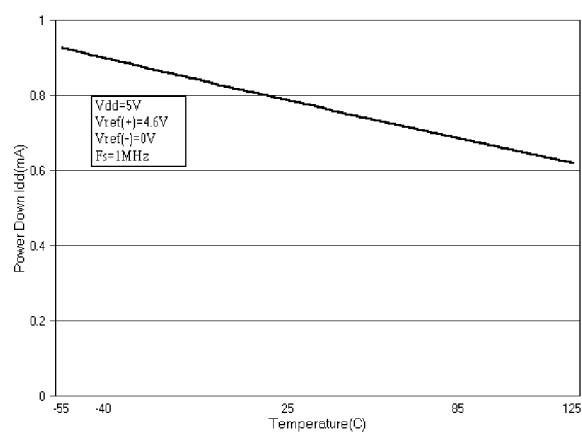
Graph 8. Power Down Current vs. Temperature
