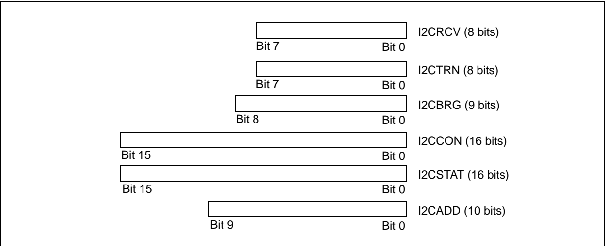
FIGURE 15-1: PROGRAMMER’S MODEL
