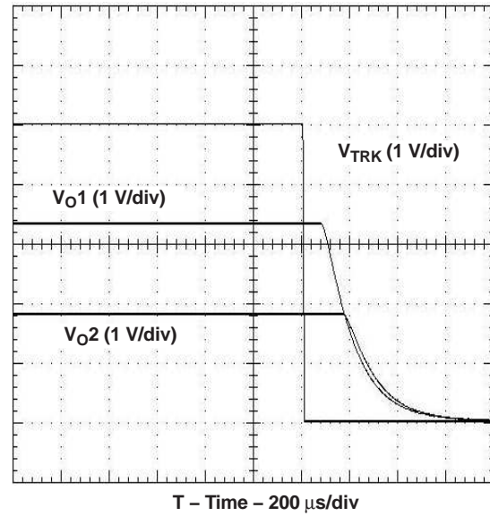
Figure 26. Simultaneous Power Down With Auto-Track Control
