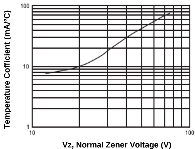
Fig.3-Temperature Coefficients
