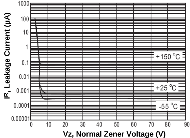
Fig.4-Typical Leakage Current
