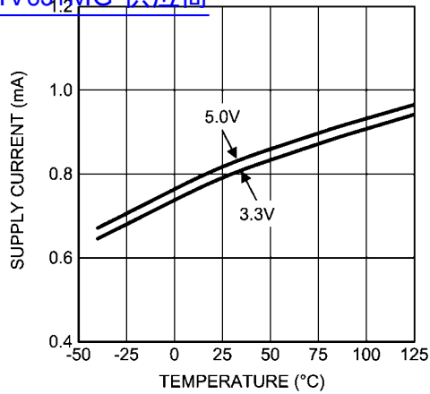
Supply Current vs. Temperature Dual LMV852 查询"LMV851MG"供应商
