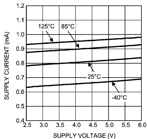
Supply Current vs. Supply Voltage Dual LMV852
