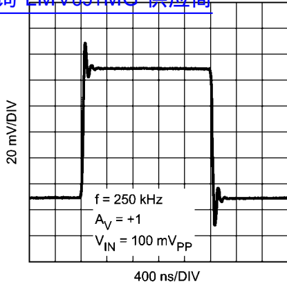
Small Signal Step Response with Gain = 1 查询"LMV851MG"供应商
