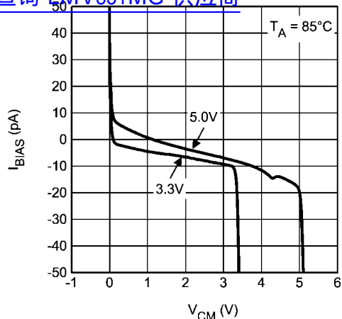
Input Bias Current vs. V_{CM} at 85°C 查询"LMV851MG"供应商
