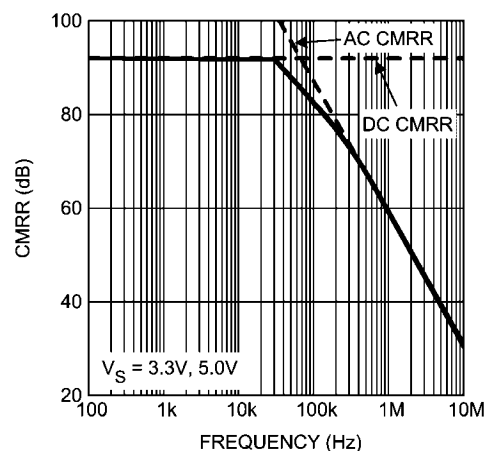
FIGURE 2. CMRR Curve
