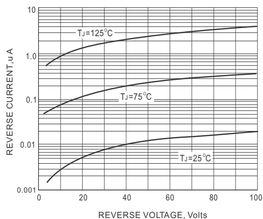
FIG. 2-TYPICAL REVERSE CHARACTERISTICS
