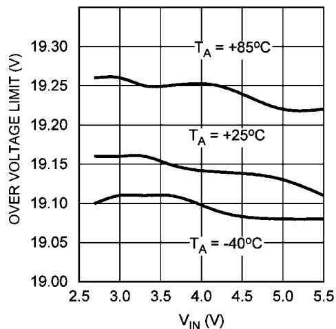
Over Voltage Limit vs V_{IN} ( V_{OUT} Rising)
