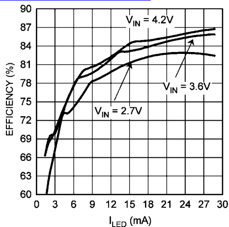
2 LED Efficiency vs I_{LED} ( V_{IN} = 4.2V , V_{OUT} = 12V , R_L = 0.66\Omega )
