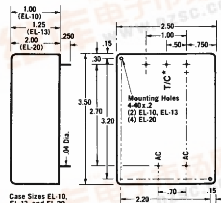
Case Sizes EL-10, EL-13, and EL-20.
