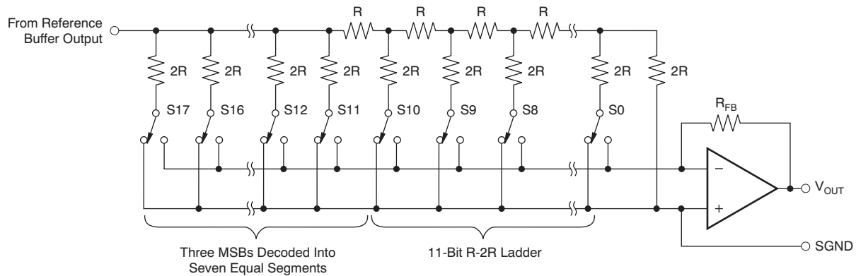
Figure 41. DAC8234 Architecture
