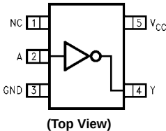
Pad Assignments for MicroPak
